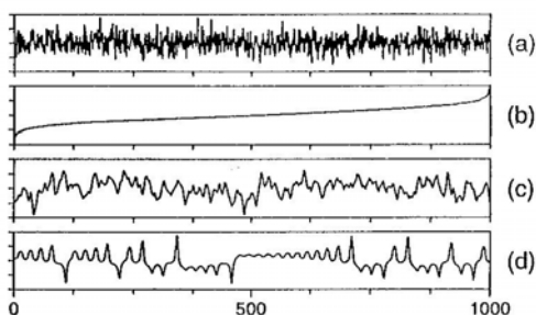
FIG 6. Example of four synthesized time series with identical means, standard deviations, and ranges. Series (c) and (d) also have identical autocorrelation functions and therefore identical power spectra. Reprinted with permission. 39
